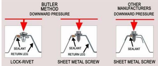
Sealant and return leg guarantee roof performance (Source: Butler manufacturing product literature; http://www.butlermfg.com/images/level3_pages/returnleglink-large.jpg visited 5/23/06).
