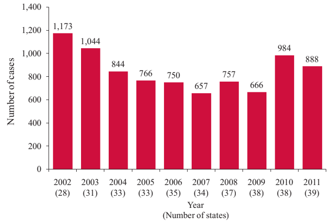
36b. Number of cases of BLLs \geq 25 \mu\text{g}/\text{dL} in construction, 2002-2011
