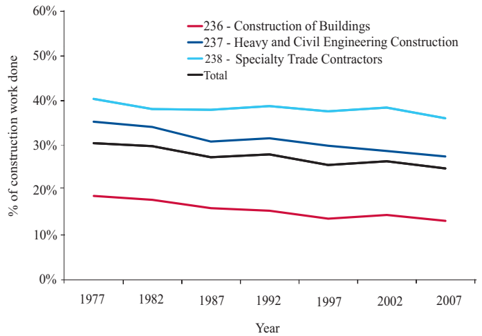
4c. Payroll and fringe benefits as a percentage of the value of construction work done, 1977-2007
