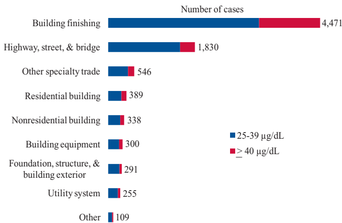
36c. Number of cases of BLLs 25-39 \mu\text{g}/\text{dL} and \geq 40 \mu\text{g}/\text{dL} , by construction subsector, 2002-2011
